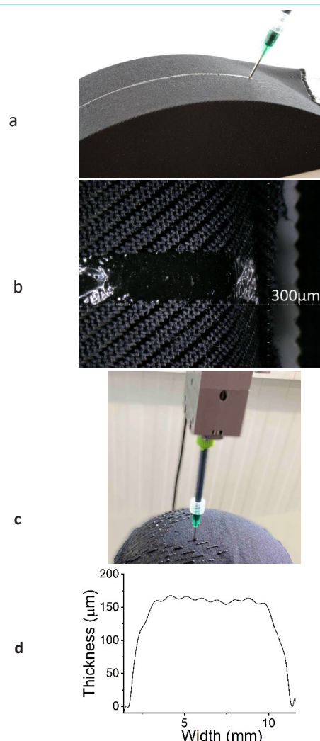
Figure 6: a) Robot-assisted dispensing process of a line on an elliptic curved gabardine textile using the Vippro head dispensing unit integrated on a UR 10 robot; b) microscopic view of the dispensed HAPTIC® ink on curved surfaces. c) Robot-assisted dispensing of TPU test structures on spherical knitted fleece fabric with its shape retaining behavior profilometry measurement of dispensed HAPTIC® onto gabardine textile with an average layer thickness of 165 µm (d).
