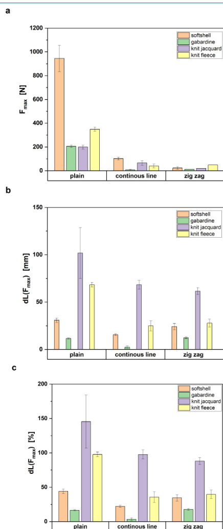
Figure 5: a) Maximum force, b) elongation, and c) relative elongation at the point of sample rupture for softshell, gabardine, knit jacquard, and knit fleece fabric.
