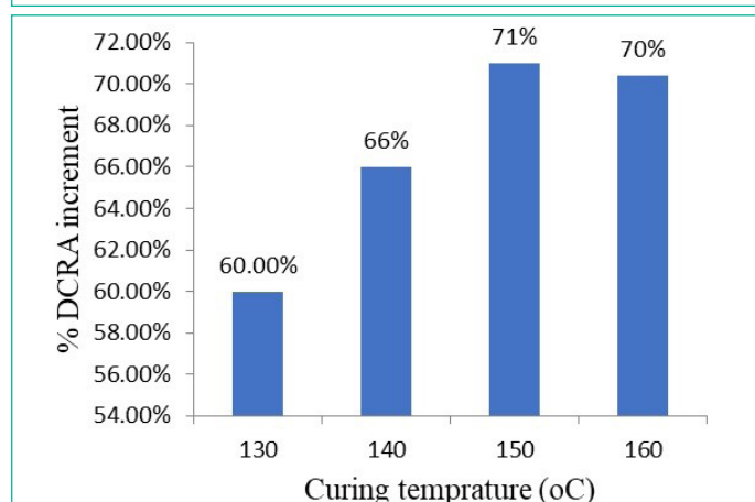
Figure 6: Effect of curing temperature on DCRA.
