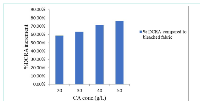
Figure 4: Effect of Citric Acid Concentration on DCRA.
