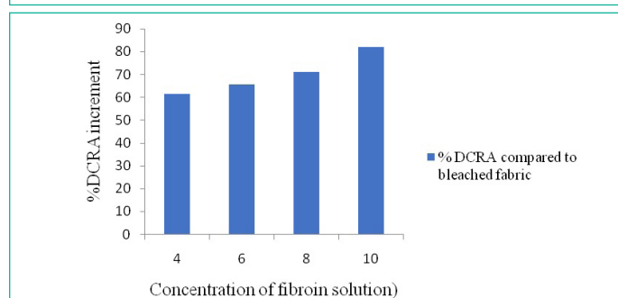
Figure 5: Effect of fibroin solution on DCRA.
