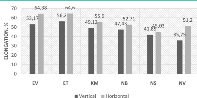
Figure 18: Elongation knitted fabrics, %.
