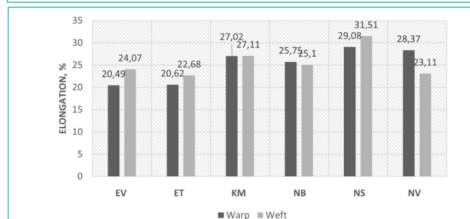
Figure 14: Elongation of woven fabrics, %.
