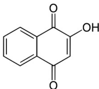
Figure 1: 2-Hydroxy-1, 4-Naphthoquinone [16].
