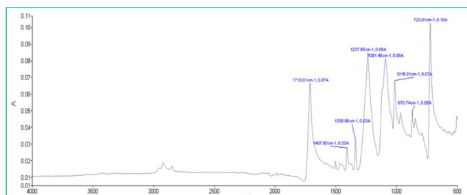
Figure 8: FTIR result of alkali treated polyester fabric.
