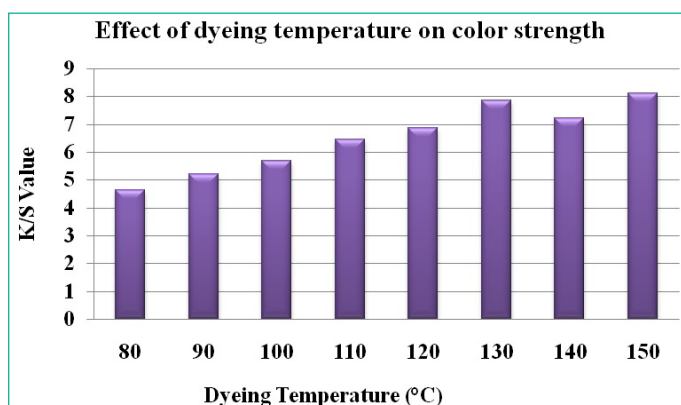
Figure 9: Effect of dyeing temperature on K/S value.
