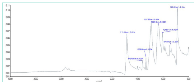
Figure 7: FTIR result of untreated polyester fabric.
