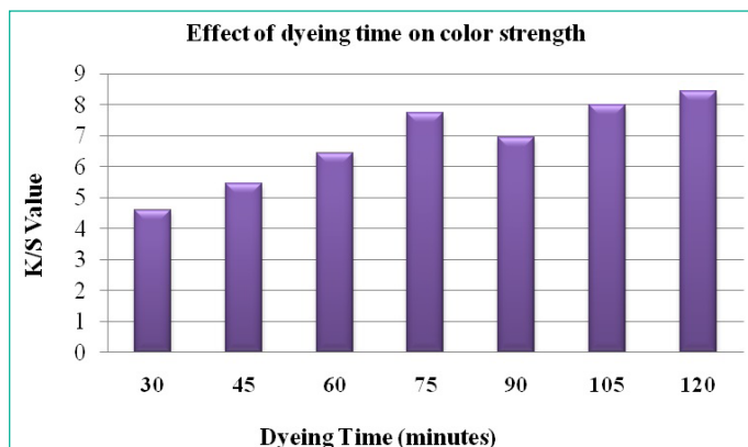
Figure 10: Effect of dyeing time on K/S value.
