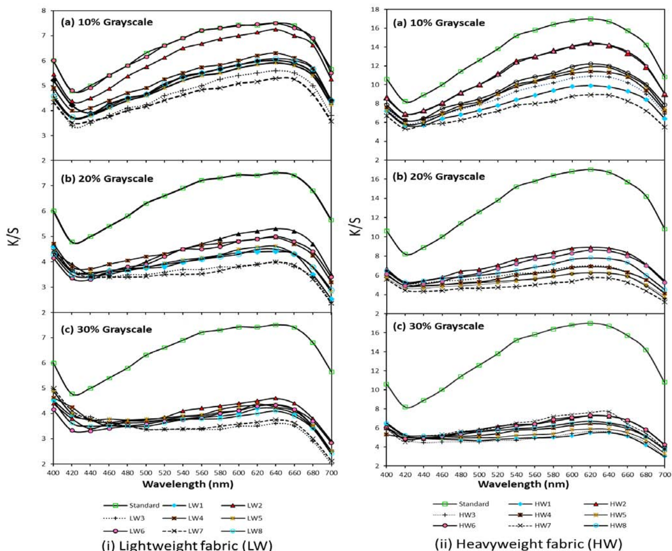
Figure 5: Spectrophotometer – colour yield (K/S) for LW and HW fabrics – 10, 20 and 30% grayscale.
