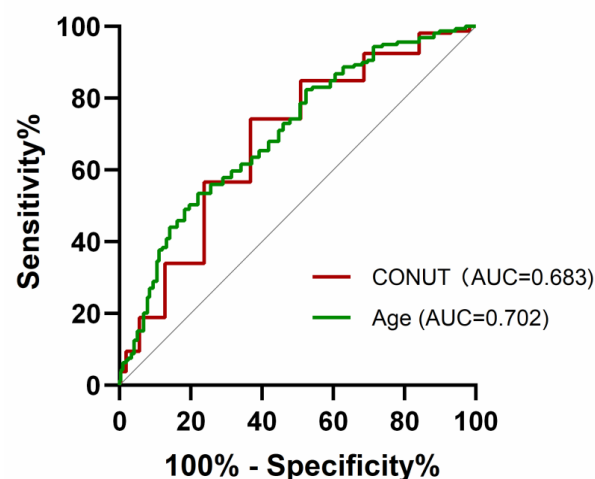
Figure 1: ROC curve of CONUT score and age predicting cardiovascular events in MHD patients.
