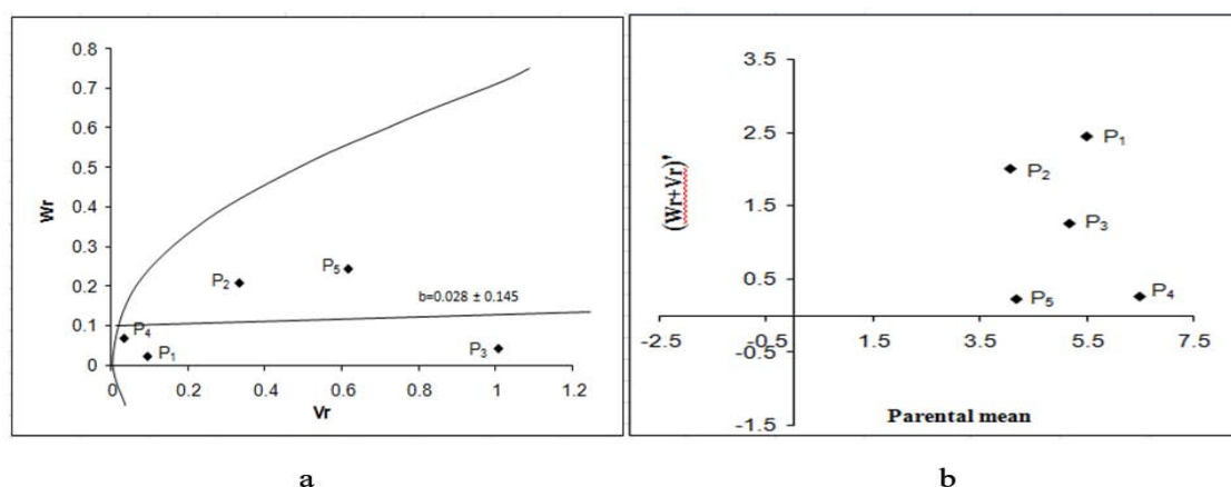
Figure 10: V_r-W_r graphs (a) and W_r+V_r /parental mean graph (b) for total sugar.
