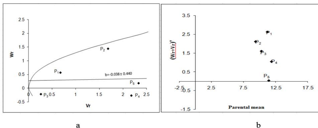
Figure 3: Vr-Wr graphs (a) and Wr+Vr/parental mean graph (b) for hollowiness.
