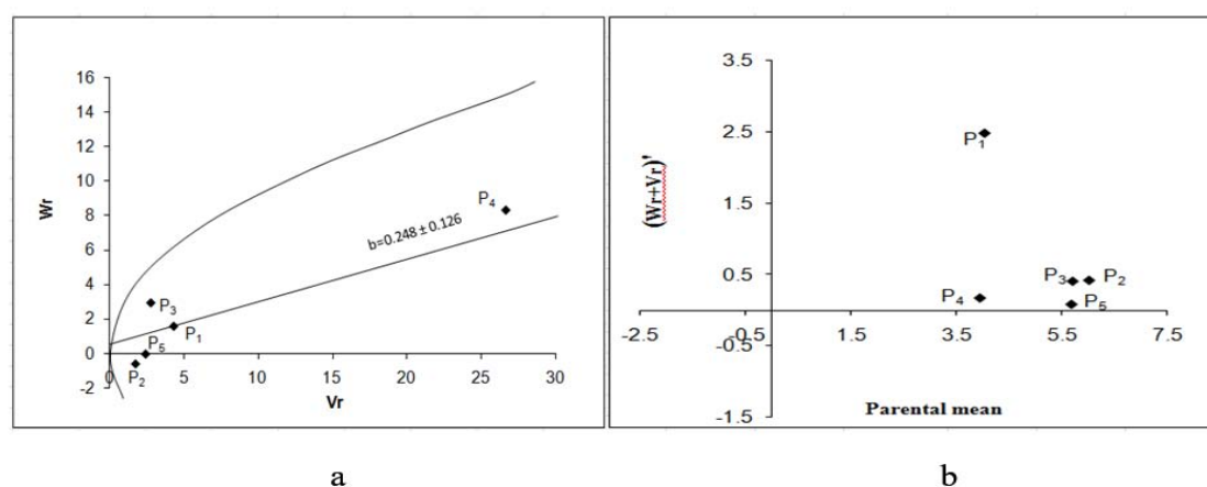
Figure 1: V-Wr graphs (a) and Vr+Vr/parental mean graph (b) for fruit length.
