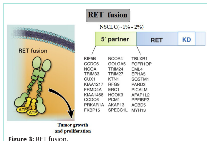
Figure 3: RET fusion.
