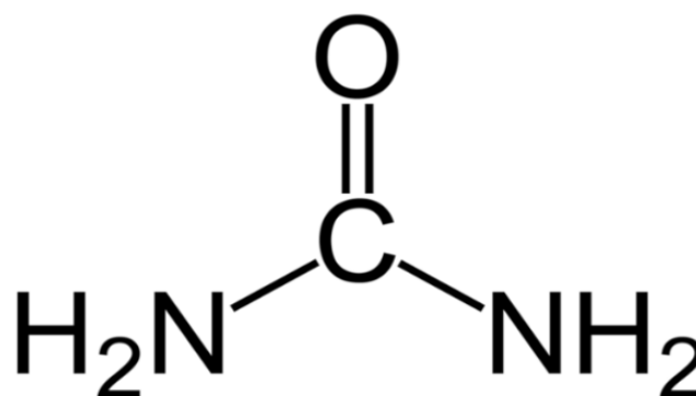
Figure 1: Urea Molecule.
