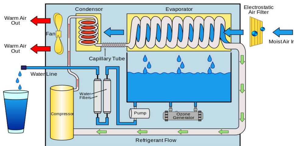
Figure 1: Air Water Generator system.
