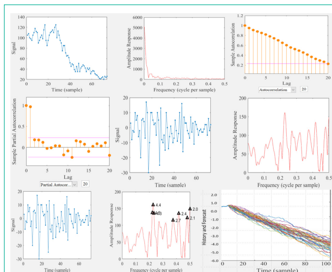
Figure 2: ARIMA/SARIMA model outputs: Sweden.
