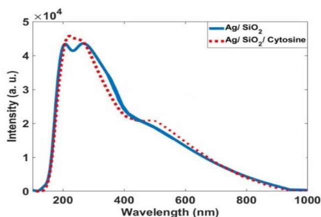
Figure 9: Calculated absorption spectra for the Ag/SiO 2 and Ag/SiO 2 -Cytosine.
