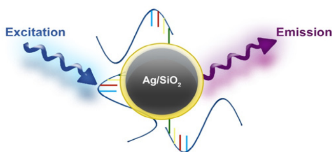
Scheme 1: FRET in RNA-Ag/SiO 2 conjugate.
