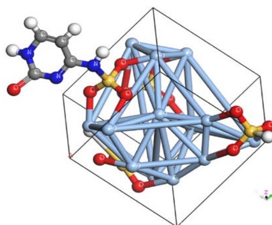
Scheme 2: DFT-calculated optimized cells of Ag/SiO 2 conjugated with Cytosine molecule.
