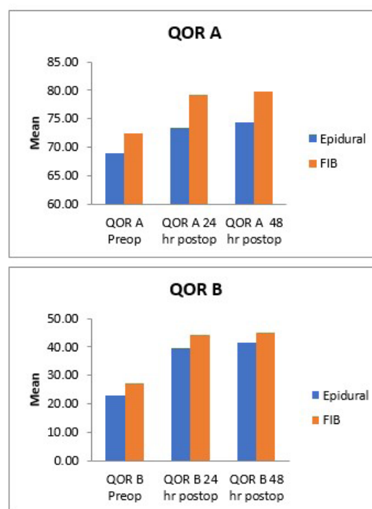
Figure 2: QOR comparison.
