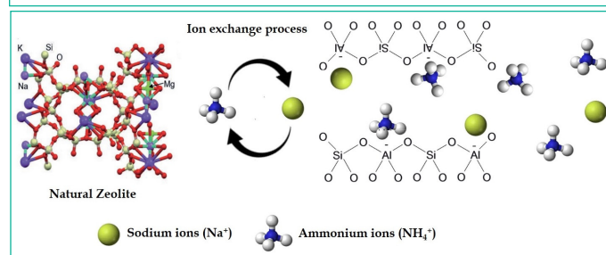
Figure 2: Mechanism of ion exchange process responsible for slow release of ammonium ions from zeolite.
