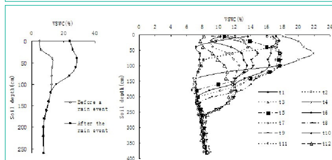
Figure 2: Two-curve method for estimating maximal infiltration depth. A: infiltration depth and soil water supply for one rain event. B: the maximal infiltration depth is estimated by a series of two-curve methods in the semiarid loess hilly region, China. VSWC is Volumetric soil water content.
