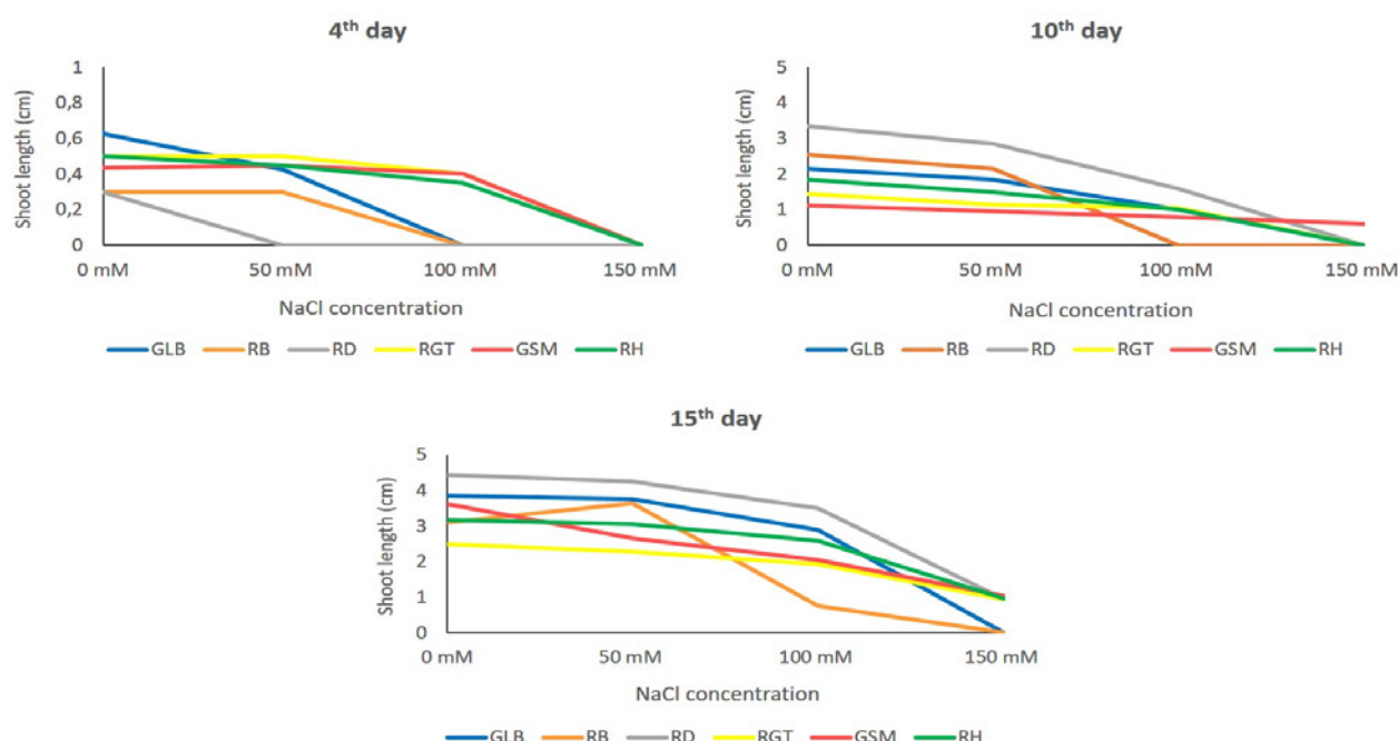
Figure 3: Shoot length (cm) of lettuce cultivars under normal and NaCl stress conditions (4 th , 10 th and 15 th day). The shoot length of RGT, RH, GSM, RD, GLB and RB at each stress level (0, 50, 100 and 150 mM NaCl) are comparatively depicted.
